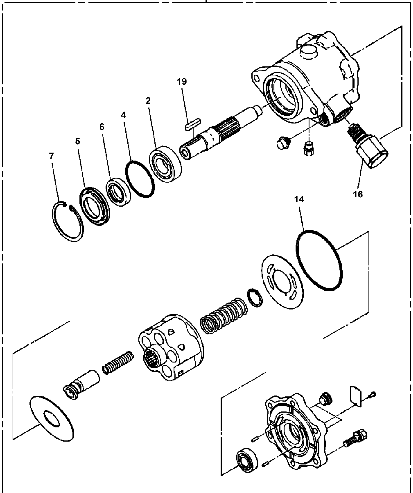
展開図有 ILLUSTRATED BREAKDOWN NO.16
