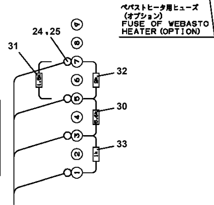
展開図有 ILLUSTRATED BREAKDOWN NO.17,24
