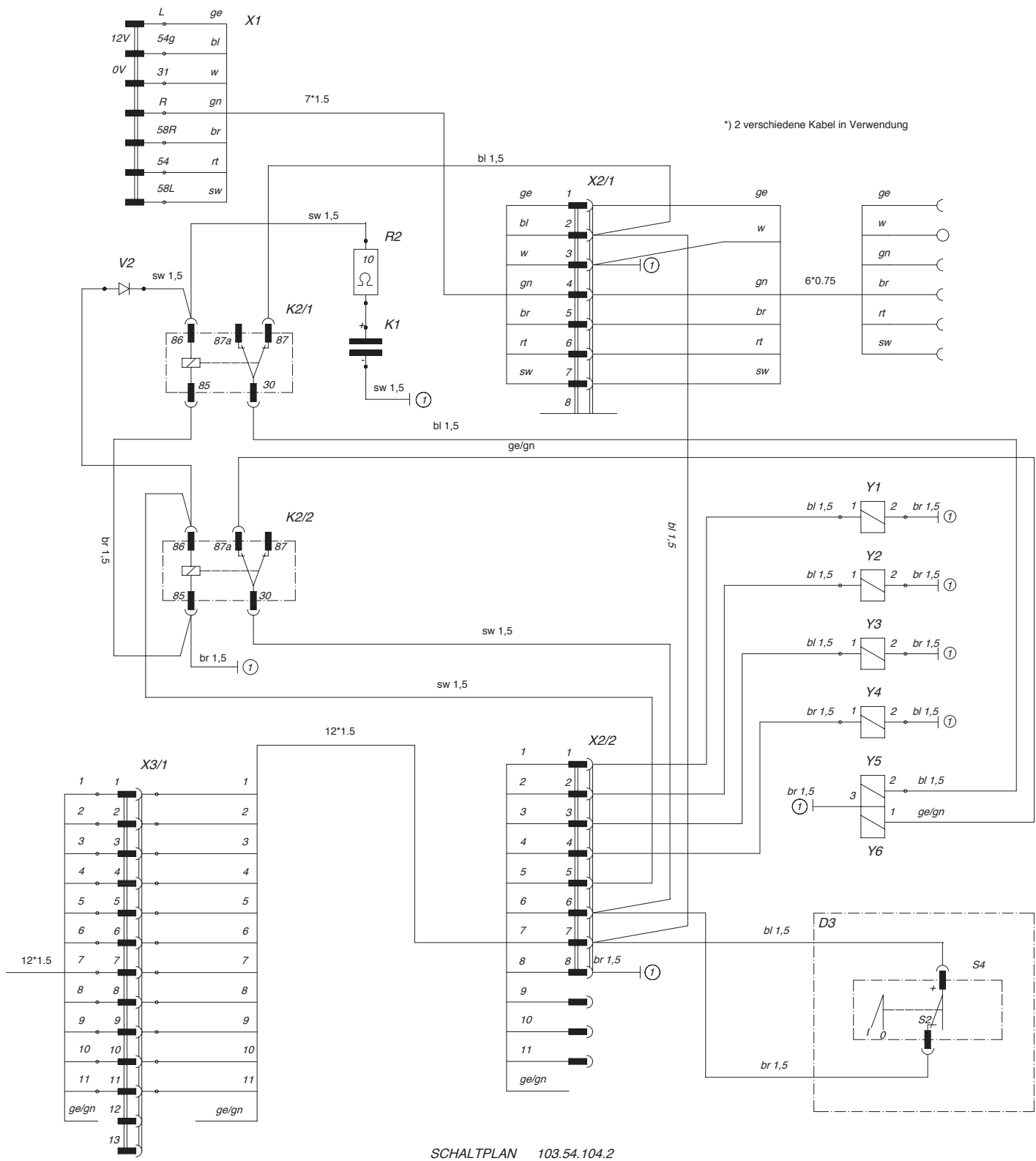
SCHALTPLAN 103.54.104.2
