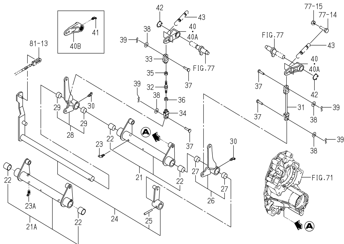
FIG. 78 PEDAL(BRAKE)SYSTEM(2/2) (EXCEPT H TYPE)
