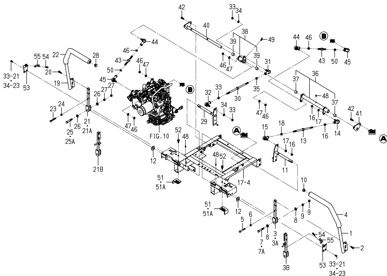
FIG. 12 LEVER(HST)SYSTEM
