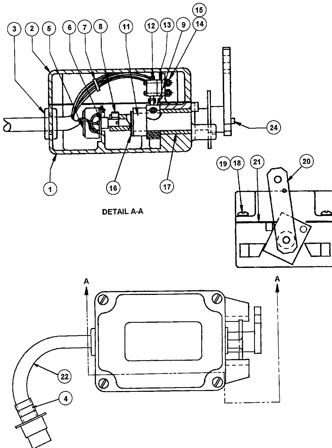
Figure 8-25: Accelerator Switch Assembly, p/n: 17070-F
