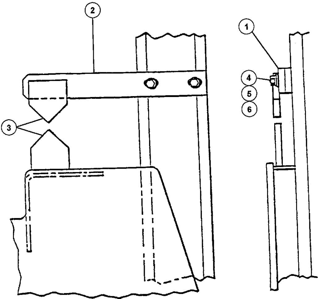
Figure 8-42: Fork/Mast Level Indicator, p/n: 36560
