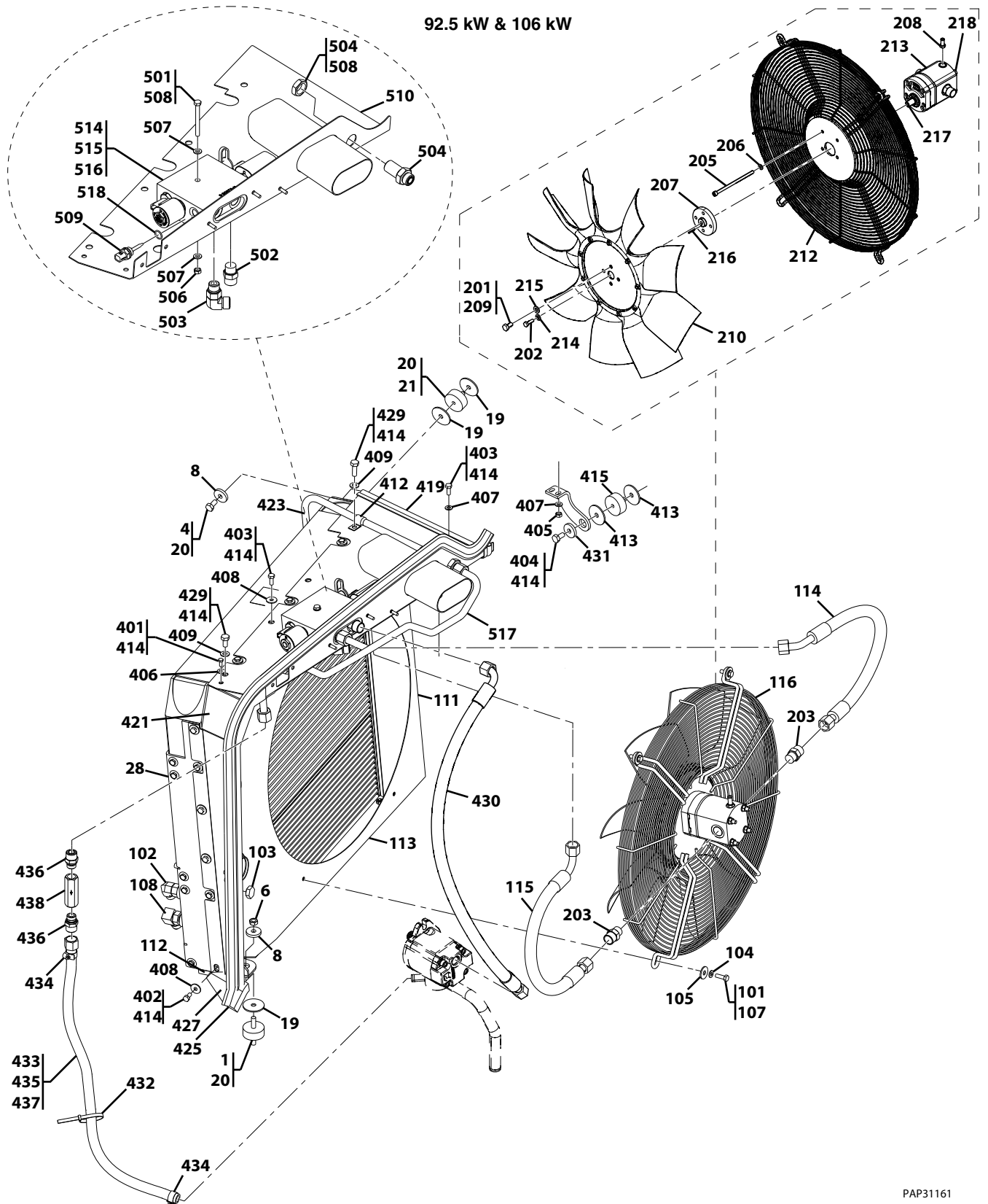
Figure 4-5 Radiator Installation (Continued)
