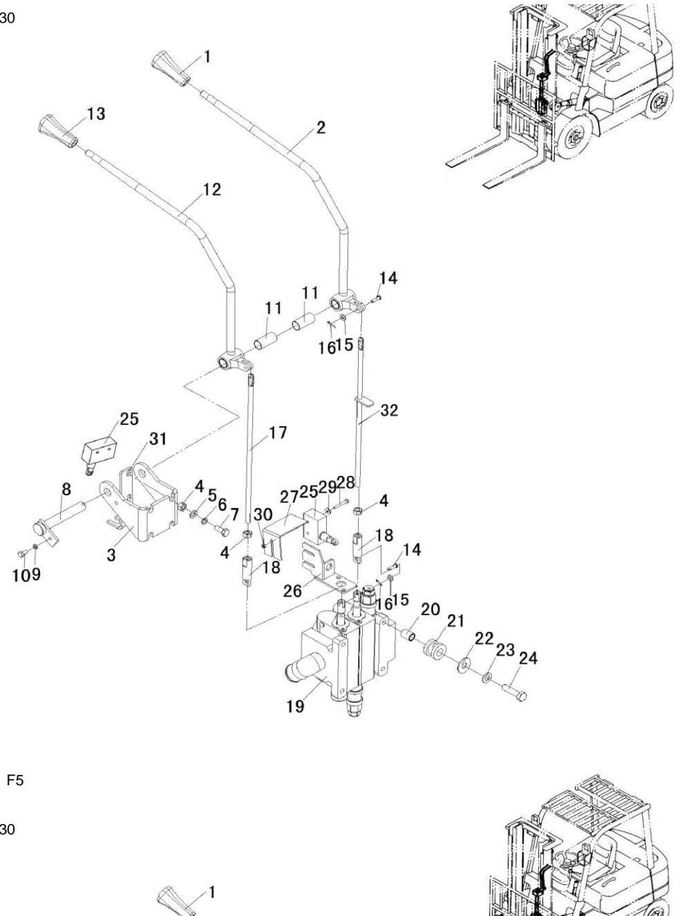
图73/FIG73 操纵杆总成(二片)/VALVE CONTROL LINKAGE(TWO-THROW)
