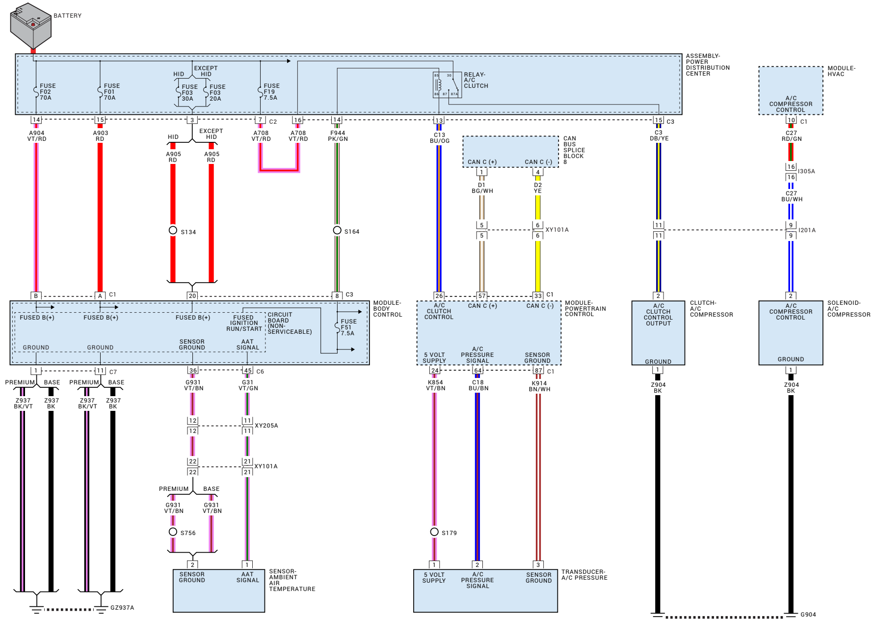
A/C CONTROL SYSTEM - 2.4L
