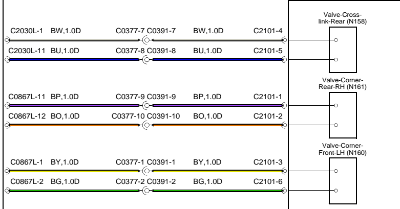
Sensor-Height-Front-RH (T238)
