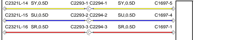
Sensor-Height-Rear-RH (T237)
